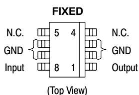
SOIC-8 D SUFFIX CASE 751
