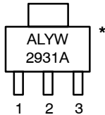
SOT-223 ST SUFFIX CASE 318H
