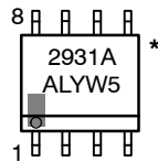
SOIC-8 D SUFFIX CASE 751
